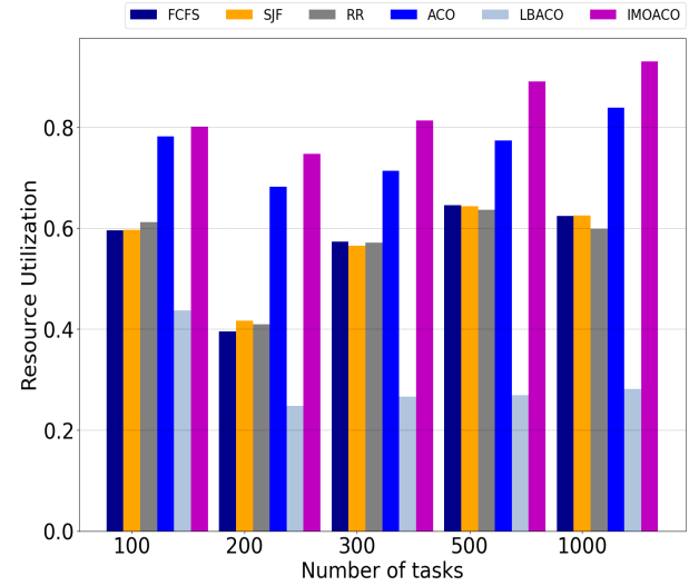
Figure 3: Comparison of resource utilization performances
