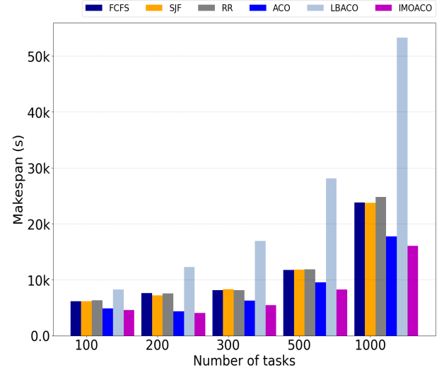
Figure 2: Comparison of makespan performances
