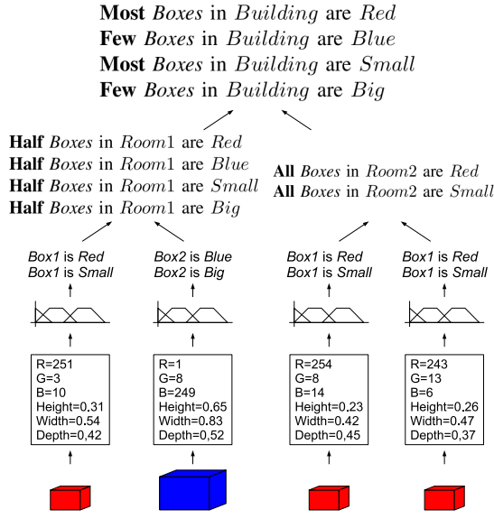
Figure 6: An example of the obtained perceptions.
