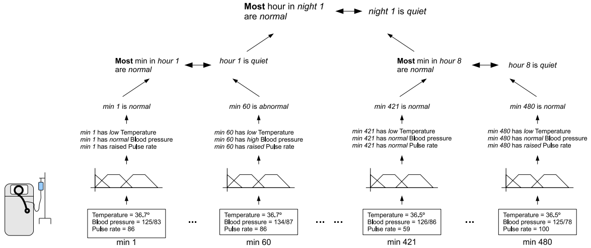
Figure 1: An example of the hierarchy.
