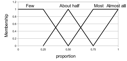
Figure 4: Fuzzy sets describing quantifiers.
