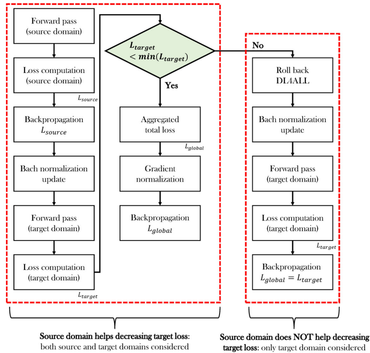
FIGURE 3: Outline of a single iteration of the proposed greedy cross-dataset transfer learning procedure: after the forward pass in the source domain, we backpropagate the loss of the source domain and compute the target loss. If the resulting target loss is reduced with respect to the previous iteration of the algorithm after considering the source domain (source domain helps decreasing target loss), we keep the model and backpropagate the target loss as well, otherwise (source domain does not help decreasing target loss) we roll back DL4ALL and consider only the target domain.
