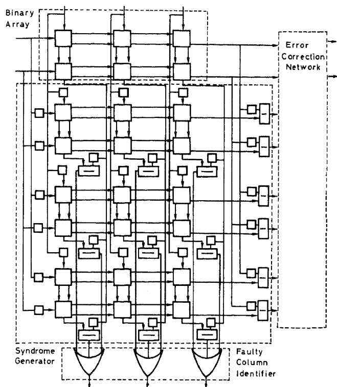
Fig. 7 - Bidimensional array with fault localization
