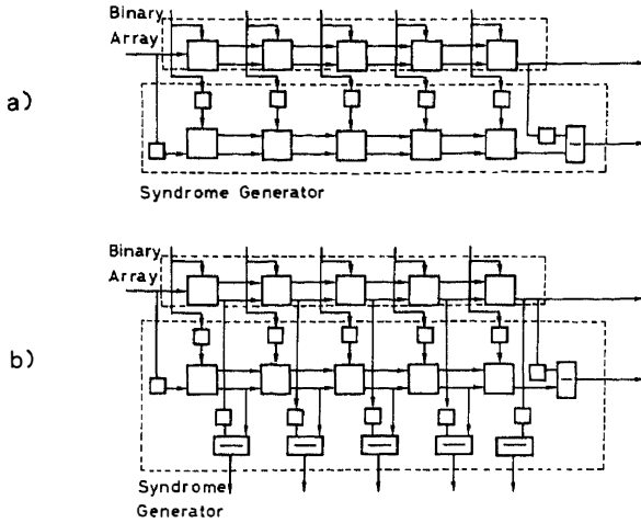
Fig. 9 - Single error detection in linear array
