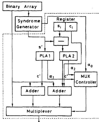
Fig. 11 - Correction generator for single-syndrome consecutive errors
