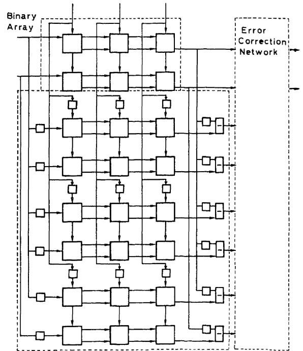
Fig. 6 - Fault-tolerant bidimensional array
