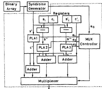
Fig. 12 - Correction generator for double-syndrome consecutive errors
