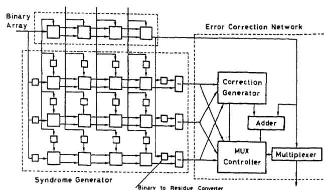
Fig. 4 - Fault-tolerant linear array
