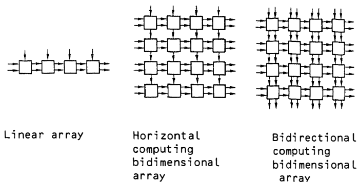
Fig. 3 - Different topologies for arrays
