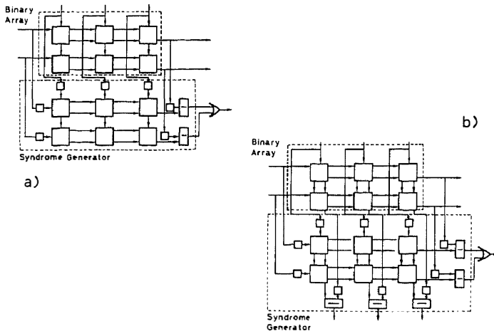
Fig. 10 - Single error detection in bidimensional arrays
