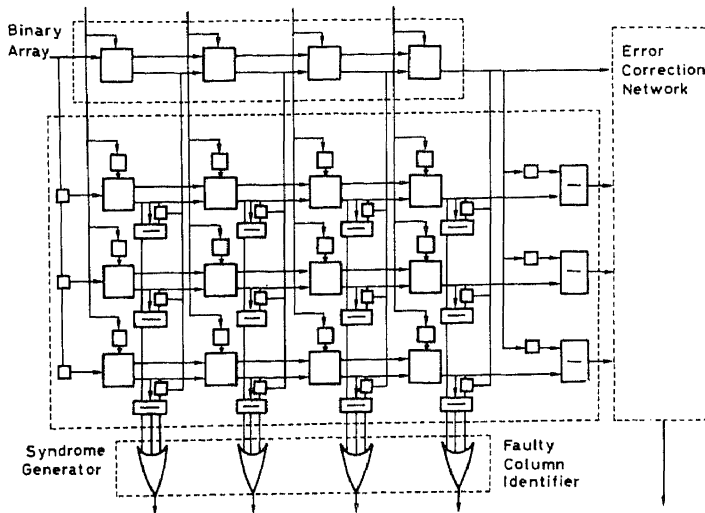
Fig. 5 - Linear array with fault localization
