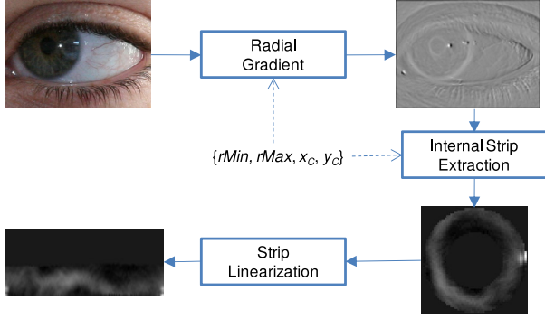
Fig. 3. Step B.1: ROI extraction. The agent extracts a linerized strip of the radial gradient image around the current position of the agent \{x_C, y_C\} .
