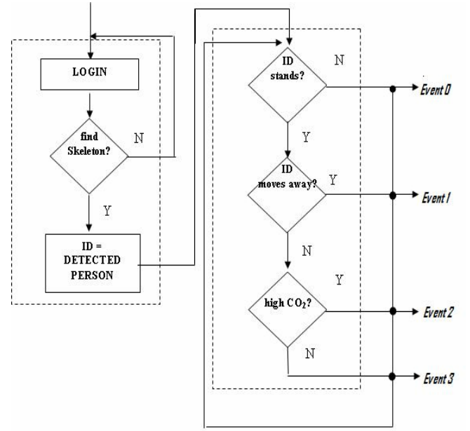
Figure 2: flowchart representing the logical steps of a simple version of the implemented human presence detection system
