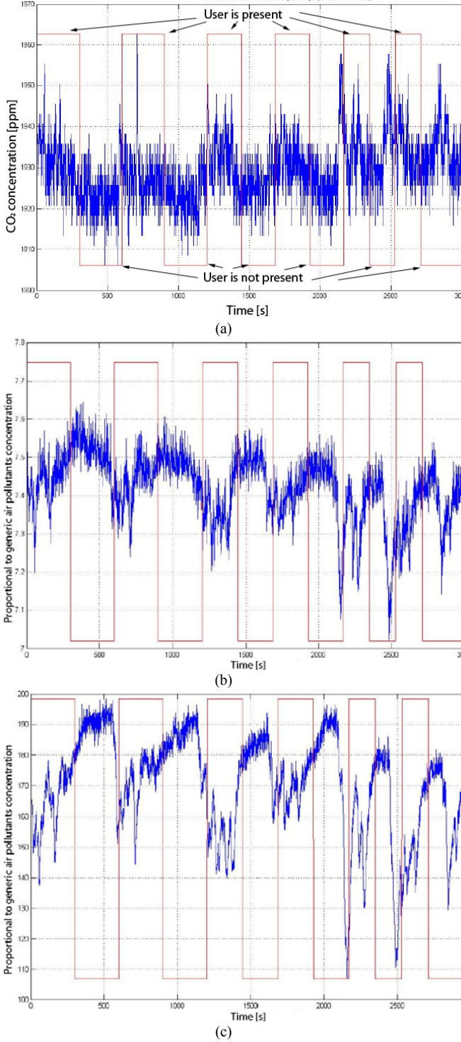
Figure 3 - An example of sensor response to human presence. This diagram is referred to the sensor Figaro TGS-4161 (a) that is sensible to \text{CO}_2 , TGS-2442 (b) and TGS-2600 (c) that are sensible to various air pollutants.
