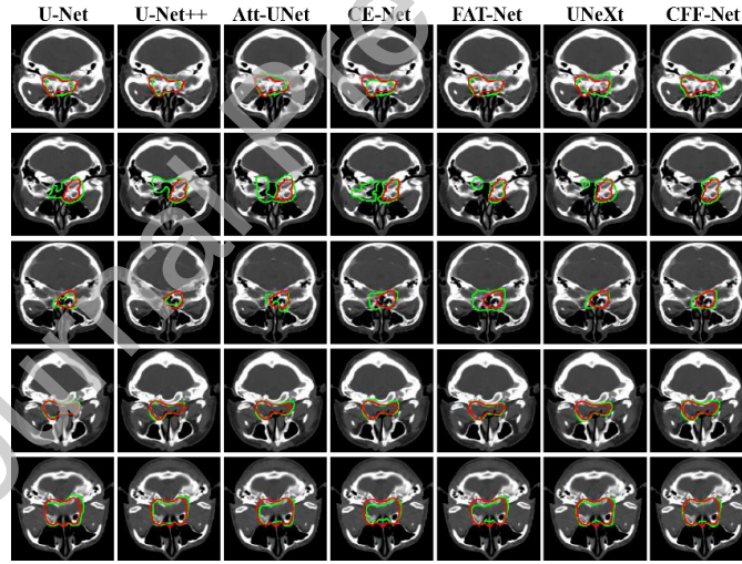
Fig. 13. Visualization of the comparative results of different models in the NPC dataset. The red and green contours indicate the boundaries of ground truth and segmentation predictions.
