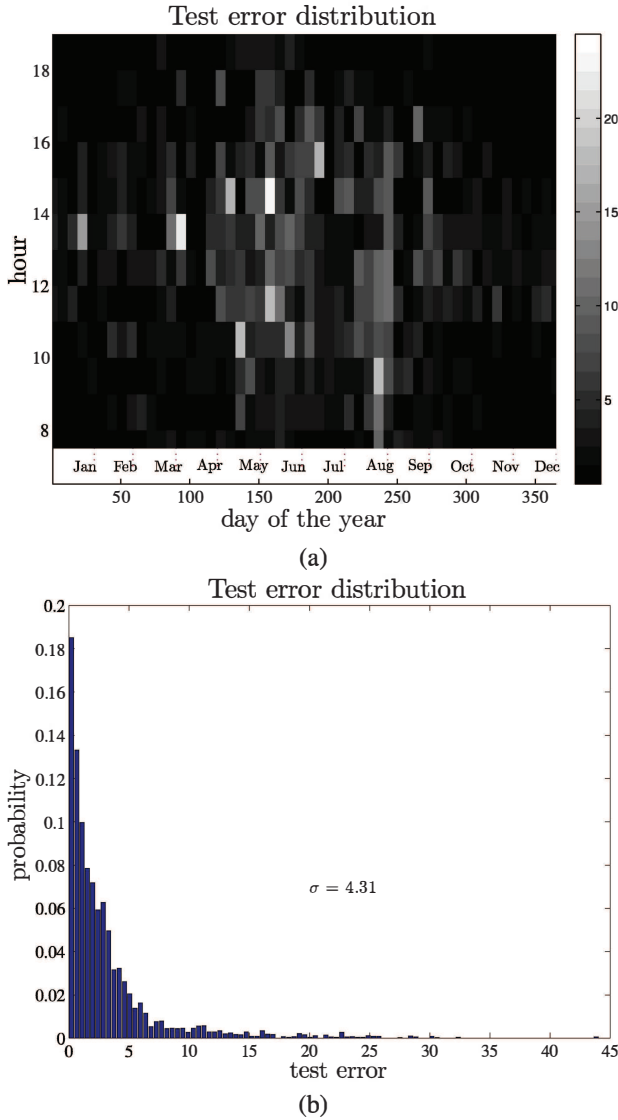
Fig. 3. Test error distribution. In panel (a), the test error computed in all the trials is reported with respect to the day of the year and the hour. Since the test set does not include all the possible time combinations, the error have been reported averaging those of seven consecutive days. The error is almost uniform on the domain, although it slightly follows the seasonal and daily variability. In panel (b), the estimated probability density function of the test error (which standard deviation is 4.31).
