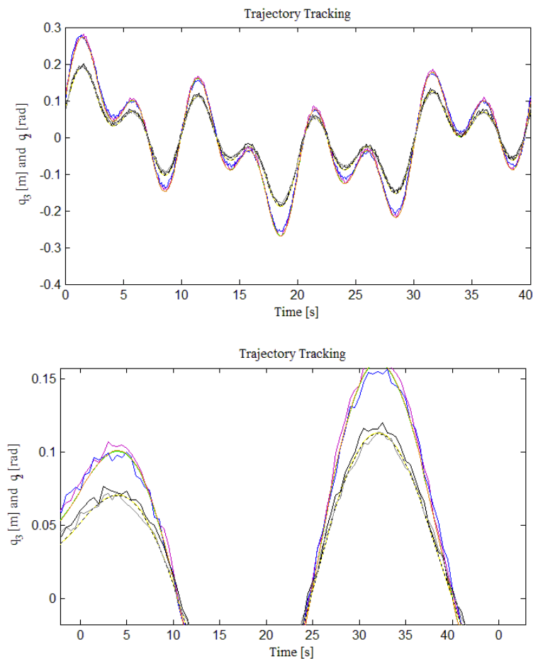
Fig. 1. Trajectory Tracking. Upper chart: nominal and simulated results. green line – reference signal for q_3[\text{m}] ; black dotted line – reference signal for q_2 . violet: q_3[\text{m}] (LM, n_h:=20 ), blue: q_3[\text{m}] (1spsa, n_h:=35 ), red: q_3[\text{m}] (2spsa, n_h:=20 ); grey: q_2[\text{rad}] (LM, n_h:=35 ), black: q_2[\text{rad}] (1spsa, n_h:=20 ), yellow: q_2[\text{rad}] (2spsa, n_h:=20 ); Lower chart: zoomed part of the upper chart.
