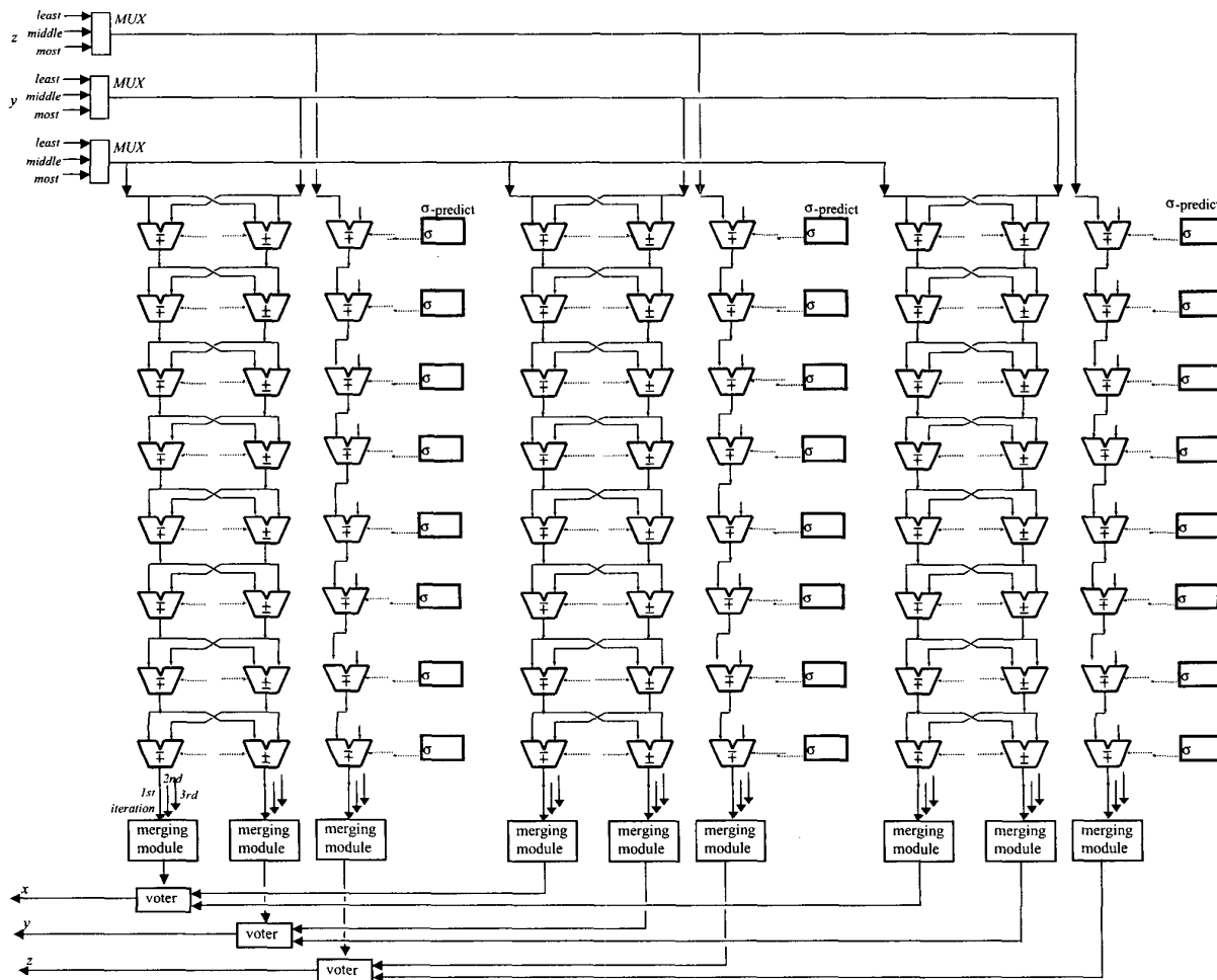
Figure 1. The CORDIC structure with concurrent error correction ability.
