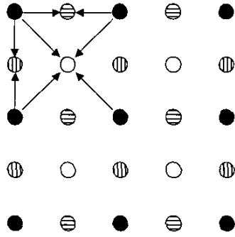
Fig. 4. Data sets. Base sampling set, B \subset R^2 , (black circles). Testing set, T \subset R^2 : testing points are located horizontally (points filled with horizontal lines), vertically (points filled with vertical lines), and diagonally (white circles). Arrows identify the base sampling points used to predict the surface height in the testing point.
