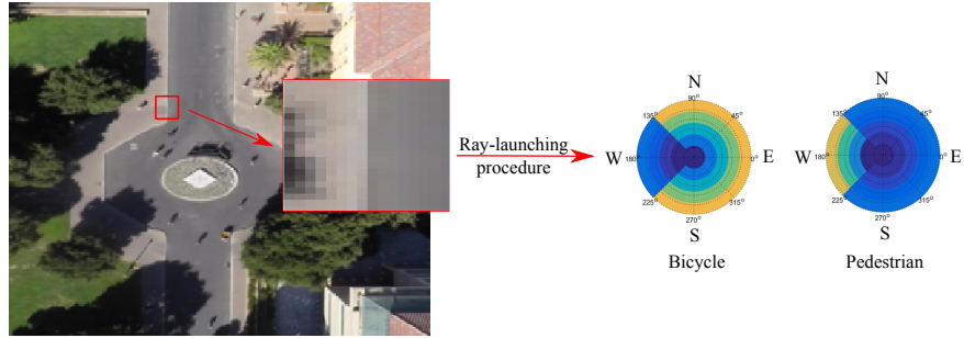
Figure 5: The figure shows the distribution S(\rho, \theta|p) for a specific location p highlighted with a red rectangle along with its magnification for two target classes. To simplify, we considered four directions for the ray-launching procedure (N, S, E, W). The distribution for the bicycle class shows increasing values up to the maximum velocity v_{max} for directions (N, E, S), while the presence of a sidewalk in the W direction determines a low likely to be taken since such class tends to prefer the street. To the contrary, the pedestrian class shows an opposed behavior since pedestrians typically move on sidewalks.
