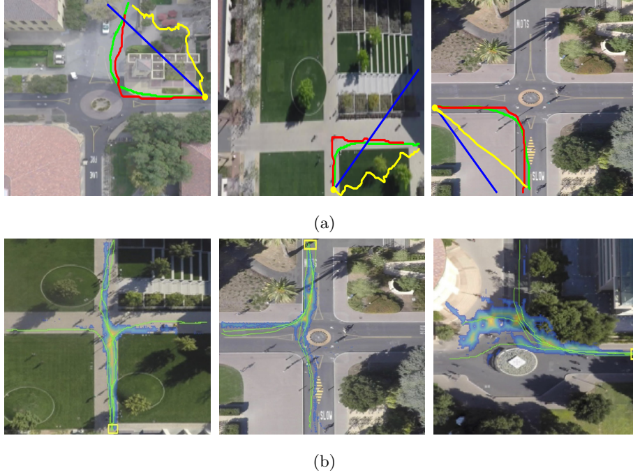
Figure 12: (a) Qualitative results for several scenarios using the CFP approach. The color code of the trajectories is the following: green = ground-truth; red = our model; blue = CV; yellow = SFM. The yellow circle represents the initial position. (b) Heat maps obtained using a uniform distribution for the Destination CD, i.e. , ignoring the final destination. We select the ground-truths, in green, as the trajectories starting from the same region highlighted with a yellow rectangle.
