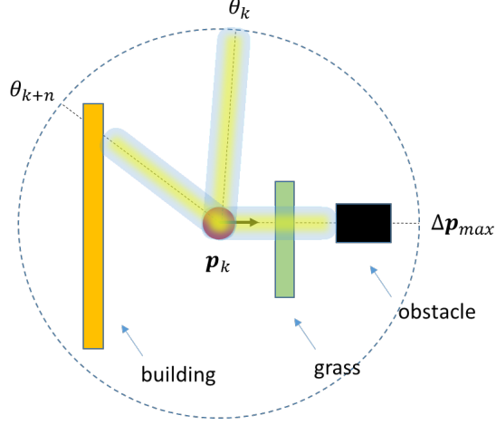
Figure 4: Illustration of the ray-launching procedure. From the pixel location p_k , a ray is launched in various directions according to the quantization defined for the model. The rays stop when either obstacles or the maximum displacement from the initial position are reached. This procedure represents the tendency of a human agent to reach free areas rather than non-free areas due to the presence of obstacles. The procedure is repeated for each pixel of the scene.
