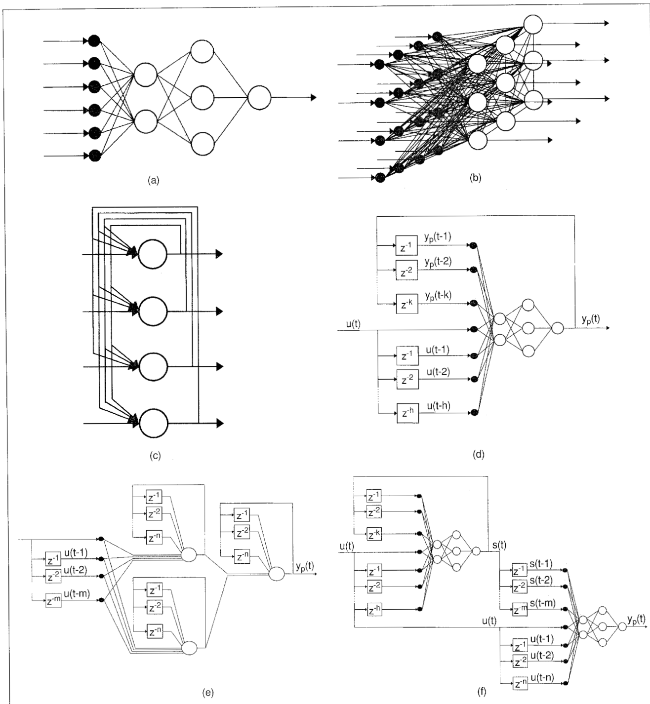
Figure 2 The neural network topologies: multilayered feed-forward (a), self-organizing maps (b), Hopfield's network (c), external feedback loops (d), local feedback loops (e), state-output network (f).
