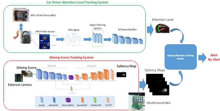
Figure 1: The overall scheme of the proposed pipeline.
