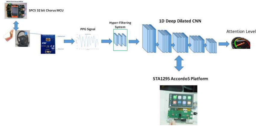
Figure 3: The proposed driver drowsiness monitoring pipeline.
