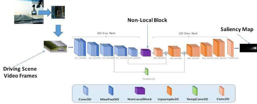
Figure 4: The proposed video saliency scene understanding block.
