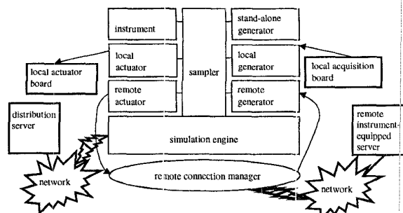
Figure 2: The client software architecture
