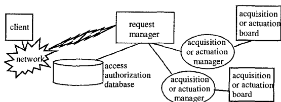
Figure 4: The software architecture of the instrument-equipped server
