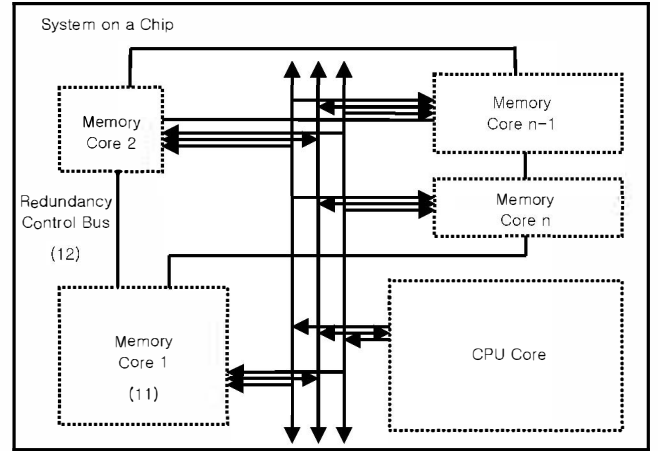
Figure 1. Typical distributed embedded memory core architecture in SoC
