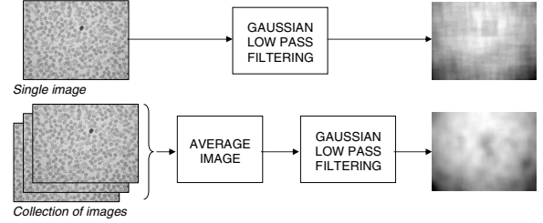
Fig. 3. Background identification by a single image (top) and by using a collection of images (bottom). Background output images are contrast enhanced to better evaluate differences.
