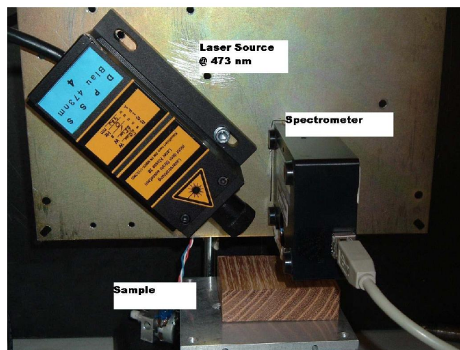
Figure1. Picture of the experimental setup: the 473 nm DPSS laser (left) excites fluorescence of wood sample (bottom right), while the miniature spectrometer above acquires the emission spectrum. The laser line is blocked by an optical long pass filter placed on the spectrometer.
