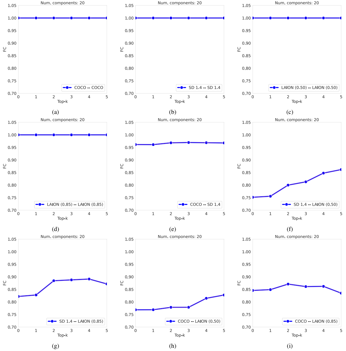
Figure 3: Similarity of the datasets used in the attack. The similarity is computed as the feature correlation (FC) on the first 20 PCA components of the image embeddings (features) for all subsets with increasing content scores. In all comparisons (panels (a)–(i)), the FC score remains relatively constant, indicating that the subsets are quite similar to each other in the feature space. Panels (a)–(d) show the similarity of random partitions of the same datasets, averaged over 10 random splits. Since the FC values are close to 1, the sets are coherent, and their images are highly similar. Panel (e) compares the COCO and SD sets (the non-member images and the images generated from their captions). The FC is slightly smaller than 1 but greater than 0.95, confirming that their contents are related. Panels (f)–(i) compare COCO or SD with the member sets, LAION-0.50 and LAION-0.85. Although the FC values remain large (never below 0.7), they are noticeably smaller than the FC values between COCO and SD (in panel (e)), suggesting a slight difference between the member and non-member images.
