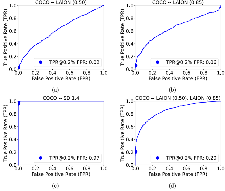
Figure 4: ROC of the attack models.
