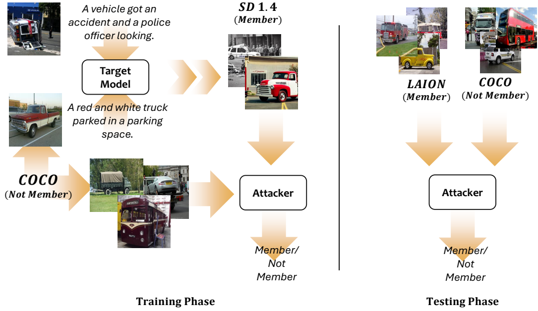
Figure 1: Attack scheme used as case study. The captions of non-member images (COCO) are used to generate the positive examples (SD-1.4) for training the attack model by querying the target model. The trained attack model is then tested using LAION images as positive examples.
