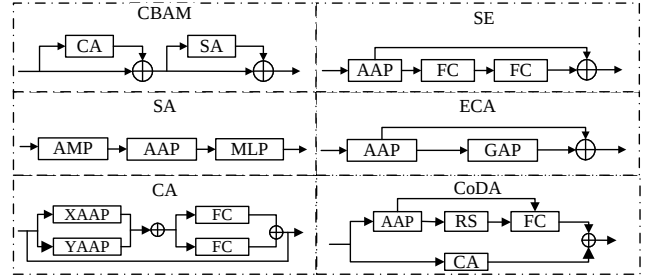
Fig. 6. Illustrates the structural layouts of representative attention mechanisms, namely CBAM, SE, ECA, SA, and CA, with the essential operations and components of each module clearly depicted.
