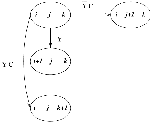
Fig. 2. States and transitions under imperfect fault-coverage.
